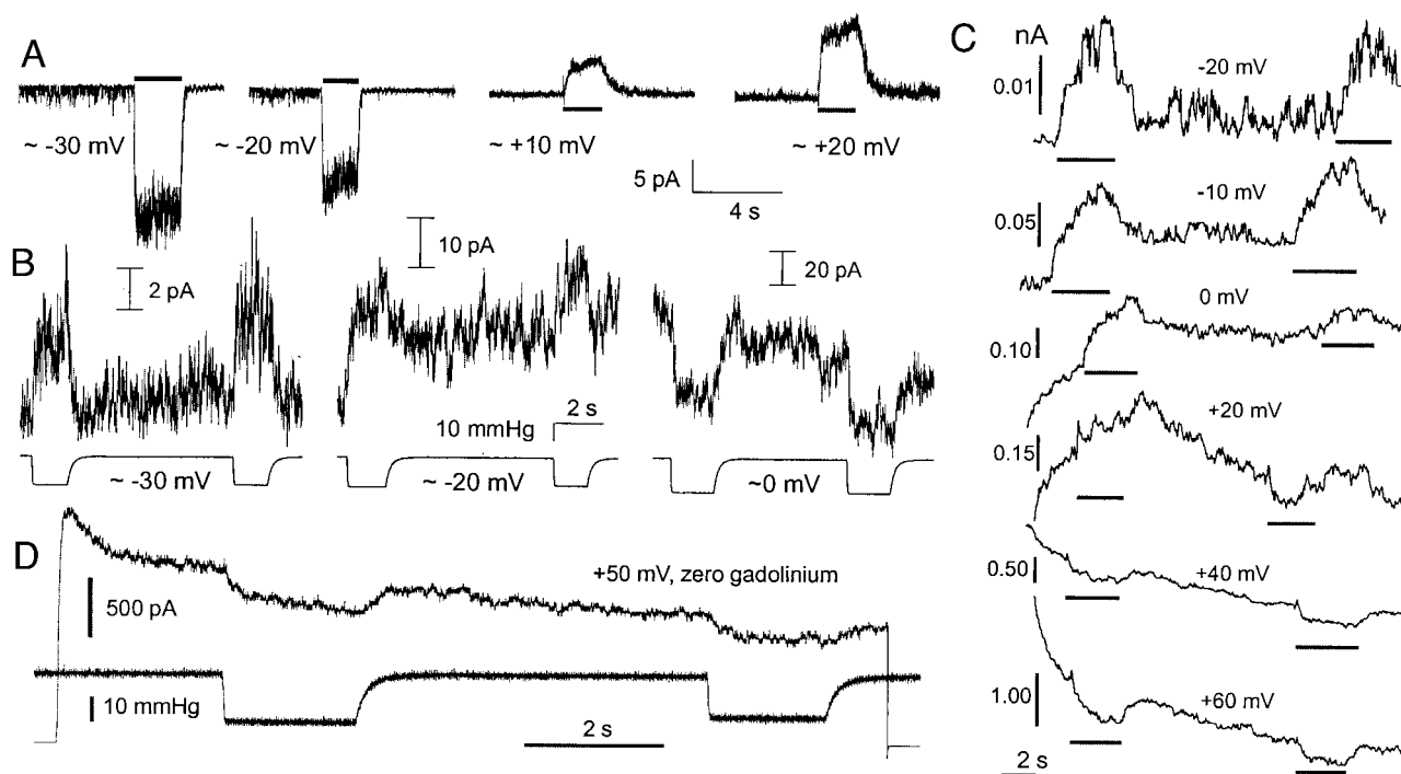
FIGURE 7 Suction effects on I_{Sh} and endogenous SA currents. ( a ) Endogenous SA I_{cation} elicited by suction of -20 mmHg (bars); cell-attached patch, noninjected oocyte, V_m as indicated, no Gd^{3+} . ( b ) Cell-attached patch clamp trace, Gd^{3+} in the pipette, Shaker -IR injected oocyte. Pipette pressure traces are below the current traces; downward deflection indicates negative pressure (suction), V_m as indicated. In the last current trace, slow (C-type) inactivation of I_{Sh} is evident. Note each current trace has its own scale. ( c ) Excised patch clamp trace, Gd^{3+} in the pipette, Shaker -IR-injected oocyte, suction ( -15 mmHg) applied as indicated by bars. Again, each trace has its own scale. Pronounced C-type inactivation of I_{Sh} is evident in the last two traces. ( d ) Excised patch, with zero Gd^{3+} in the pipette, Shaker -IR-injected oocyte (traces as in ( b ), except that current is shown at -100 mV, then +50 mV, then -100 mV, and the pressure and current traces overlap).
