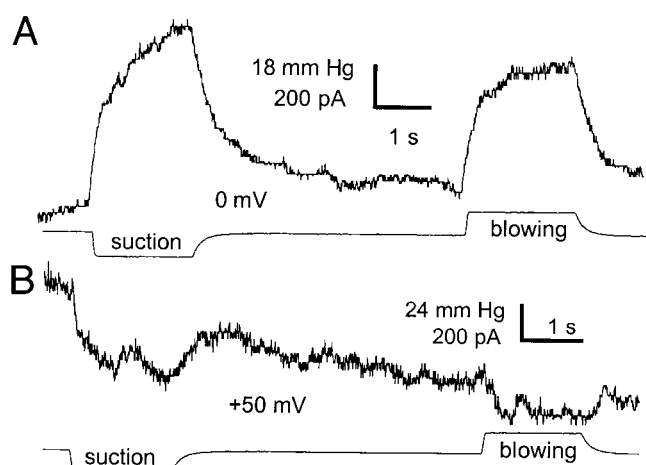
FIGURE 8 Suction and blowing have equivalent effects. I_{\text{Sh}} in two excised patches ( a and b ), V_m as indicated, and patch tension generated using both concave patch (suction) and convex patch (blowing) configurations. The pressure traces are shown below each current trace. C-type inactivation is evident in ( b ).
