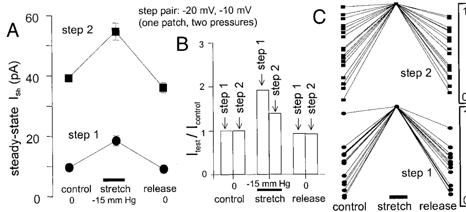
FIGURE 4 Voltage-tension interactions; analysis of step pair data. (a) From a sample patch (different patch, but raw data as illustrated in Fig. 3, b--d ), steady-state I_{sh} (mean \pm SD, n = 6 ) elicited by step 1 and by step 2 for pipette pressures 0 and -15 mmHg, before (control, "0"), during (stretch, " -15 mmHg"), and after (release, "0") mechanical stimulation. V_{command} for steps 1 and 2 was -20 mV and -10 mV, respectively. Here and elsewhere, steady-state I_{sh} was obtained by cursor measurement (Clampfit from Axon Instruments' p-Clamp). The baseline was reset to the leak current level where this was evident. (b) Mean test I_{sh} (same data as (a)) replotted as ratio of the control I_{sh} for step 1 and step 2. (c) Among-patches comparisons of the relative extent of stretch-activation in 17 excised patches; here, within-patch values have been normalized by setting the mean " I_{sh} stretch" in each patch to unity. For all 17 patches, the step pair was -20 mV, -10 mV, and in most patches stretch was elicited by -10 mmHg suction. Paired t -tests (step 1 [ I_{stretch}/I_{control} ] versus step 2 [ I_{stretch}/I_{control} ]) in each patch showed that the fold-increase nearer the foot of G(V) exceeded that for 10 mV more depolarized ( p < 0.01 ).
