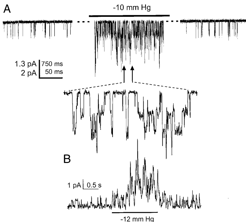
FIGURE 2 Endogenous SA cation channel events and SA events from a Shaker -IR-injected oocyte. (a) Single-channel recording of endogenous MS cation channel events from a control oocyte (cell-attached patch; no \text{Gd}^{3+} ; V_m = \sim -50 mV) before, during (including expanded section), and after the indicated pipette suction. (b) Cell-attached patch-clamp recording ( V_m = \sim -20 mV) from Shaker -IR-injected oocyte in the presence of \text{Gd}^{3+} , showing steady-state outward unitary current events, then sustained (and reversible) stretch-activation during pipette suction.
