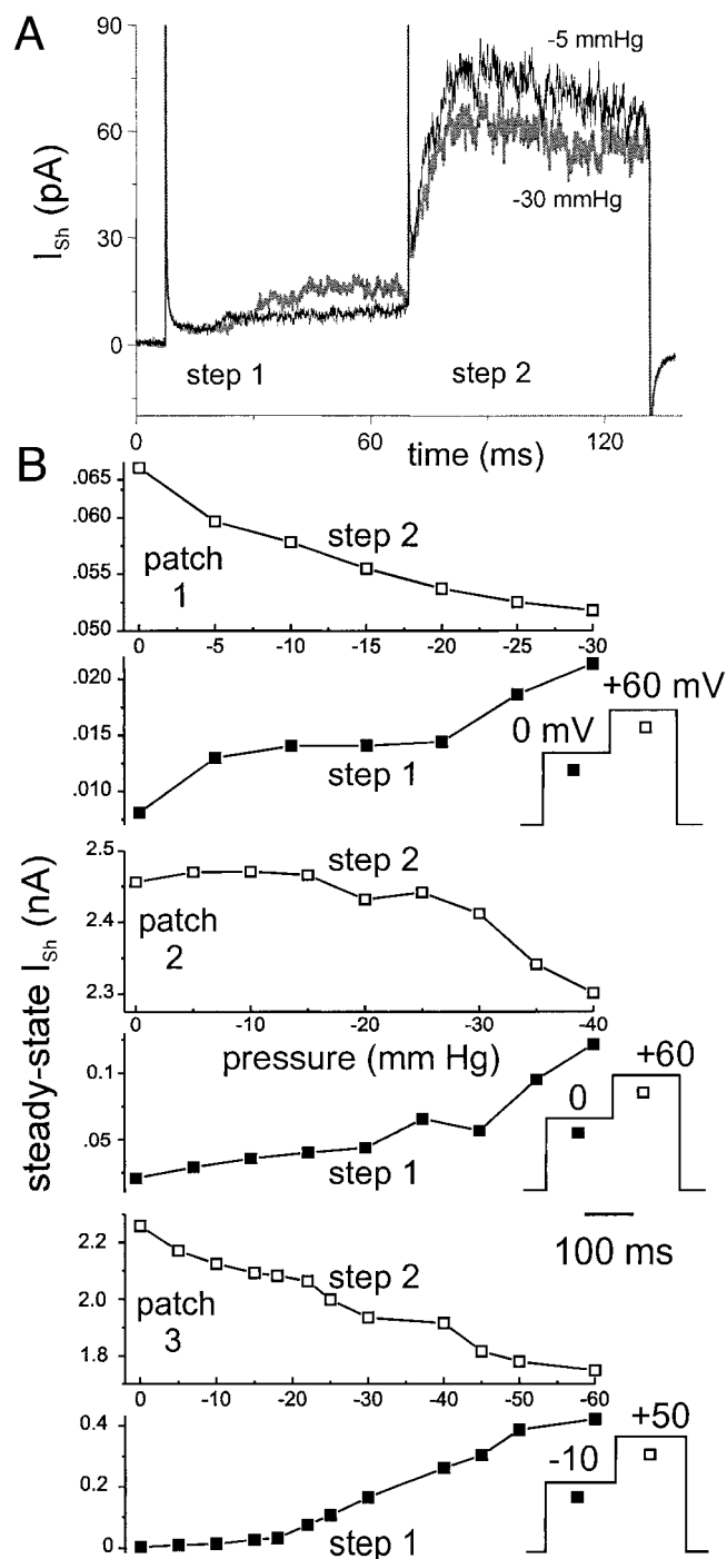
FIGURE 6 Within-patch pressure dose-responses for “foot-to-head” step pairs. ( a ) Raw step pair currents from patch 1 (see ( b )) at two different test pressures. ( b ) Steady-state I_{Sh} from three excised patches using 60-mV step pairs at the indicated voltages. I_{Sh} magnitudes differed greatly 60 mV apart and so are plotted separately with different y axis gains. The particular step pair for each patch is indicated (■, step 1; □, step 2).
