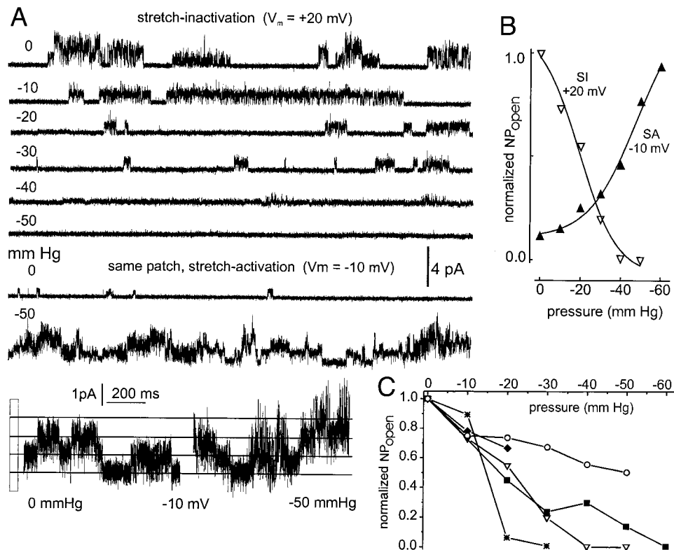
FIGURE 11 High versus low prestretch P_{open} ( V_m ), single-channel data. (a) Five-second current traces from 20-s continuous recordings, collected in the sequence shown. After the series at V_m = +20 mV, the patch was clamped at V_m = -10 mV and taken from 0 to -60 mmHg in 10 mmHg steps (not all shown). The two higher-resolution fragments of -10 mV current trace (bottom) are provided to allow for comparison of current amplitudes during periods of exceptionally high activity at 0 mmHg and of exceptionally frequent transitions at -50 mmHg. (b) SA and SI dose-responses for this patch at V_m = +20 mV ( \nabla ) and V_m = -10 mV ( \blacktriangle ) using normalized NP_{open} . The fits are for display. (c) Single-channel dose-responses (protocol as in Fig. 9, with NP_{open} calculated from 20-s recordings) from five excised patches at depolarized (elevated NP_{open} ) voltages: +60 mV (*); +40 mV (○); +60 mV (◆); +20 mV ( \nabla , same as in (b)); +60 mV (■). NP_{open} values were normalized for each patch.
