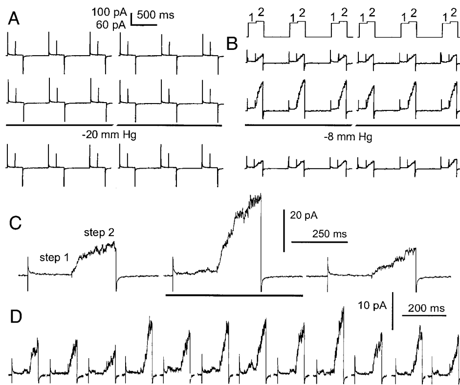
FIGURE 3 Examining SA of Shaker-IR by step pair experiments. The top right “battlement” pattern (6 step pairs labeled 1, 2) shows the V_{\text{command}} used to elicit the currents illustrated for excised patches of (a) one control and (b)–(d) three Shaker-IR -injected oocytes. Pipette solutions had 100 \mu\text{M} \text{Gd}^{3+} . V_{\text{hold}} was -100 mV and steps 1, 2 were 10 mV apart, as described in the text. Capacitance was compensated before an experiment, then not altered. The protocol was run before, during, and after membrane tension was elevated by pipette suction (solid bar); pipette suction in mmHg is indicated for (a) and (b). In (a) and (b) gaps correspond to \sim 1 s, during which the data buffer was emptied and the next run initiated ( V_{\text{hold}} and pressure were maintained); 100 pA and 60 pA correspond to (a) and (b), respectively. (c) and (d) are higher-resolution recordings (unitary events are evident in (d)) illustrating I_{\text{Sh}} elicited by step pairs before, during, and after stretch (bars: -15 and -20 mmHg in c and d, respectively); one of the six pairs is illustrated per condition for c, several in d (illustrating large stochastic variation at low NP_{\text{open}} ). In c and d most of the current at V_{\text{hold}} is omitted (hence the gaps).
