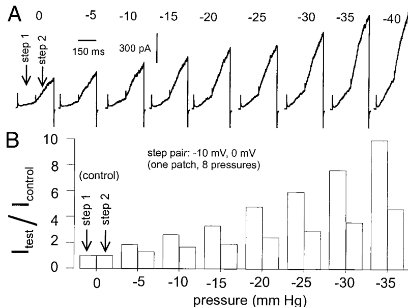
FIGURE 5 Within-patch dose-response over a wide pressure range. (a) I_{sh} traces for a step pair experiment on an excised patch with successively increasing membrane tension (pipette pressure in mmHg is indicated along the top). The step pair voltages ( -10 mV, 0 mV) were near the foot of the G(V) for the patch. The step pair was applied once/pressure. (b) The currents in (a) plotted as a dose-response using the same procedure as in Fig. 4 b (except that the step pair was applied only once at each pressure rather than six times). Since step 2 saturated the current amplifier at -40 mmHg, the plot stops at -35 mmHg.
