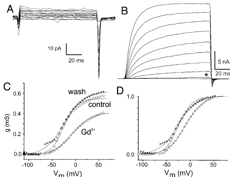
FIGURE 1 Shaker -IR currents ( I_{Sh} ) in Xenopus oocytes and effects of Gd^{3+} on I_{Sh} . Currents elicited by depolarizing steps ( -110 to +70 mV in 10 mV increments, V_{hold} = -100 mV, 1 s between successive steps) from inside-out excised patches of (a) control (uninjected), and (b) Shaker -IR cRNA-injected oocytes (asterisk below a 0 mV current trace). Electronic compensation was used to minimize initial capacitive transients. (c) Conductance-voltage ( G(V) ) curves from two-microelectrode voltage clamp for a Shaker -IR injected oocyte with control (○), 100 \mu M Gd^{3+} (△), and wash-control (*) solutions perfused into the bath. (d) Normalized version of c. The solid lines are fits to a Boltzmann equation.
