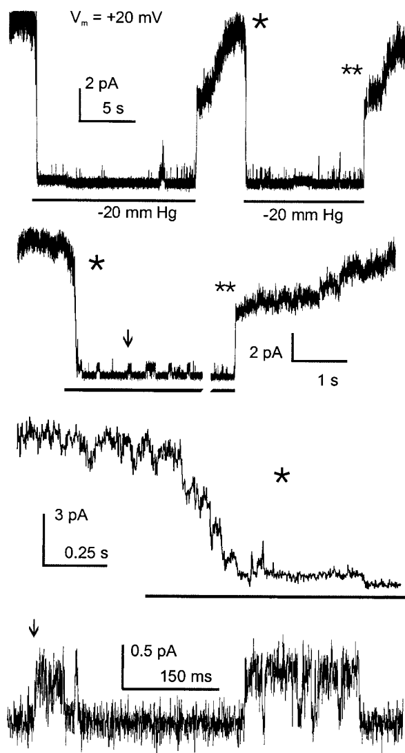
FIGURE 10 Reversible stretch-inactivation of I_{Sh} at high P_{open} . I_{Sh} from a depolarized ( V_m = +20 mV) excised patch. When suction was applied and released twice, I_{Sh} changed reversibly from a macroscopic (multichannel) to a single-channel trace. Below, this trace is seen at expanded time resolutions, with locaters provided. The trace is interrupted in the second line. Channel activity turned off via discrete current steps (third line). Suction is indicated (bar) except in the last line, when it was continuous.
